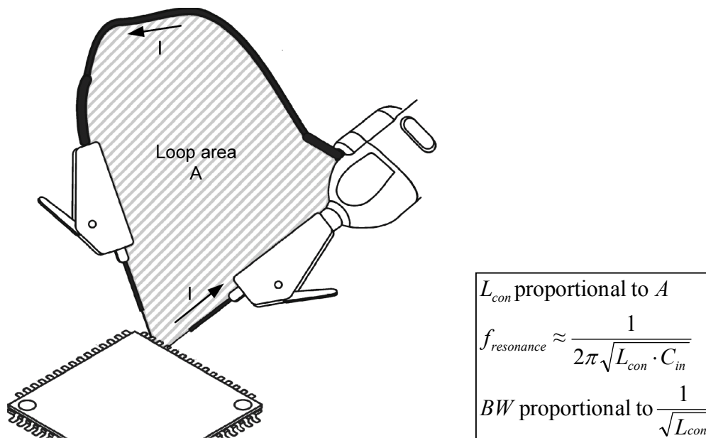
Fig. 4-4: Ground connection and connection inductance
